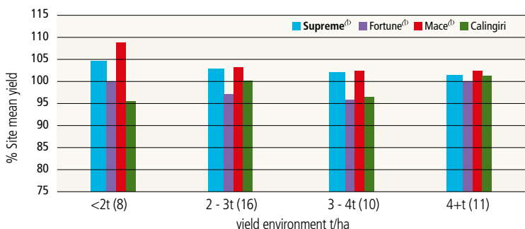
2013 WA NVT Variety performance by yield environment - represented as % of site mean yield (45 sites)
